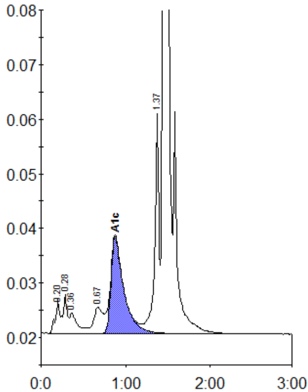
Peak table - ID: 10396362
